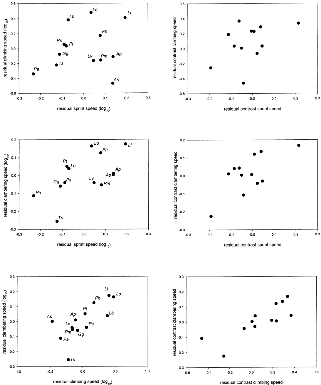
Fig. 2 Relationships among the three performance variables (sprinting, clambering and climbing speed). On the left: residuals of logarithmically transformed means per species. The point labels refer to the species (first letter of genus and species name). On the right: residuals of the phylogenetically independent contrasts.
